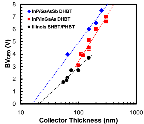
Fig. 1: BV_{CEO} vs. collector thickness for the different InP HBT material systems. As the collector is scaled, the InGaAs/InP DHBT loses its advantage over the InGaAs/InP SHBT, while the GaAsSb/InP DHBT maintains its advantage.
