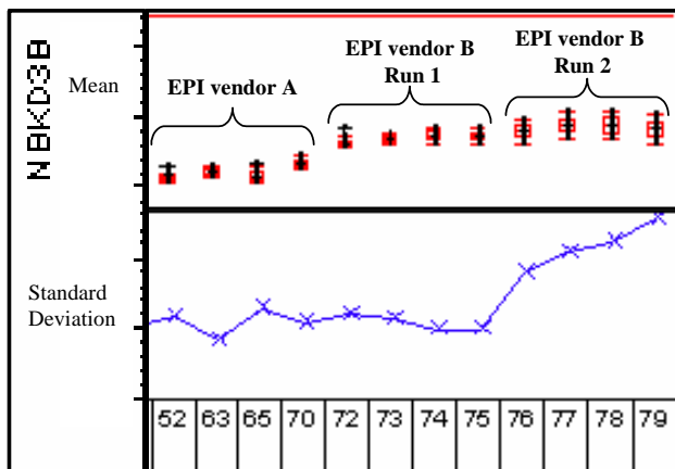
Figure 5 Plot of Nb mean and standard deviation for a group of wafers with combined NMP-based photoresist stripper and oxygen plasma. Note epi vendors can be resolved by Nb means and that individual runs between the same epi vendor are distinguishable by standard deviation.
