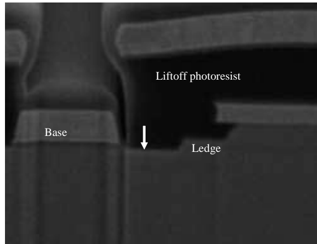
Figure 1 SEM view of HBT after base metal deposition, prior to metal liftoff. Arrow indicates GaAs surface of interest, the region between base contact and ledge epi.
