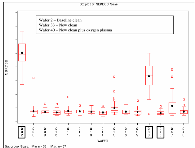
Figure 3 Nb plots of wafers with known residual photoresist from baseline cleans (wafer 2), NMP-based photoresist clean (wafer 33), and NMP-based photoresist clean plus an oxygen plasma exposure (wafer 40). Note Nb improvements with NMP-based photoresist clean and return to baseline values with the addition of oxygen plasma.
