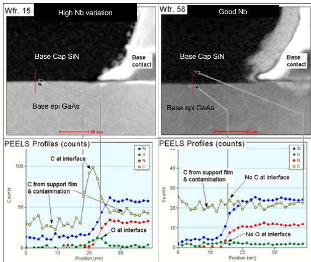
Figure 2 PEELS line scans across surface passivation-GaAs interface for a site with higher Nb (left) and a sample with historical Nb. Note carbon and oxygen are detected at the interface of the sample with higher Nb.
