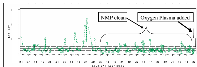
Figure 4 Device trend chart for Nb standard deviation. Note that standard deviation was improved with the NMP-based photoresist stripper and further improvement was obtained with the addition of oxygen plasma.
