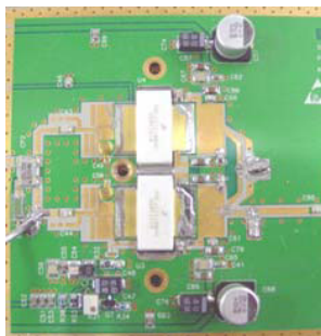
Figure 6. LDMOS Module
