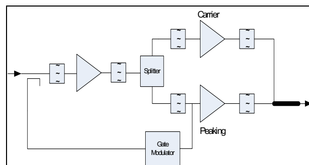
Figure 4: Doherty Amplifier with Gate Modulator and Driver
