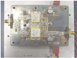
Figure 5. GaN Module
