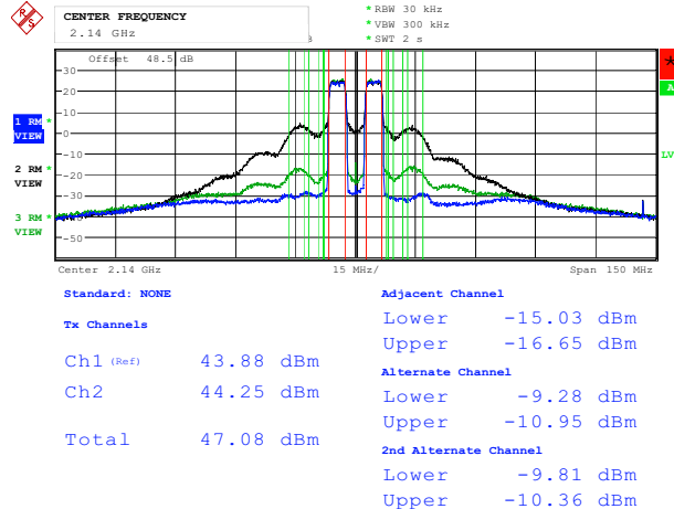
Figure 11. Spectral Measurement GaN Module 101
